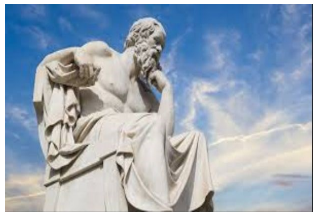
Unix Philosophy
